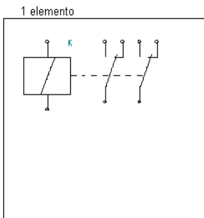
Small_RELAY-2XCLOSED DPST
