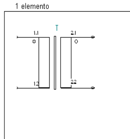
Big_TRANSFORMER-OLD-STYLE II
