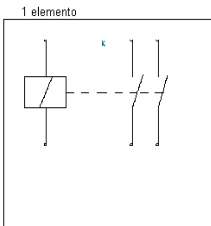
Big_RELAY-2XON DPST
